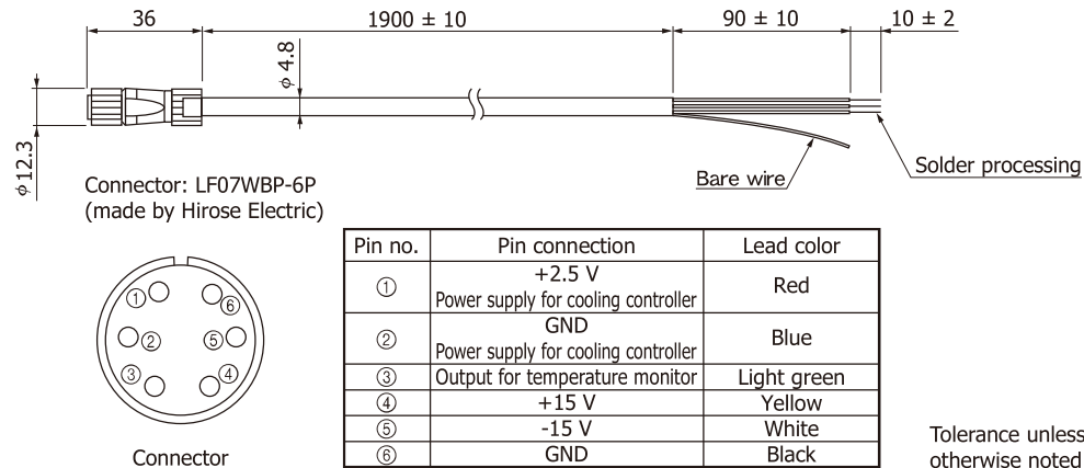
6-conductor cable (for DC power supply) A4372-07
