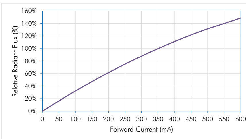
Forward Current vs. Relative Radiant Flux
