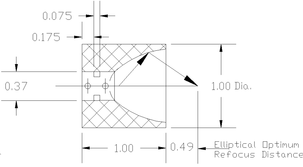
Elliptical Reflector 1" x 1"
